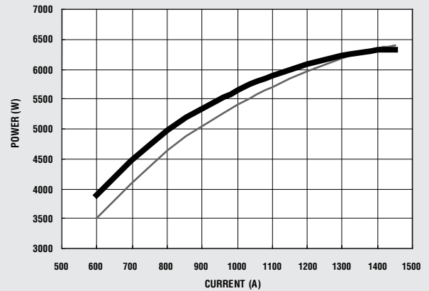
Power Performance
